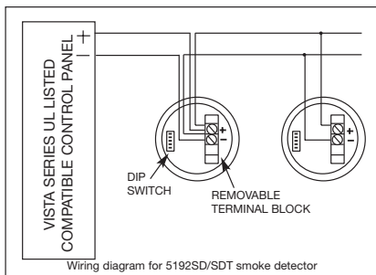
Wiring diagram for 5192SD/SDT smoke detector
